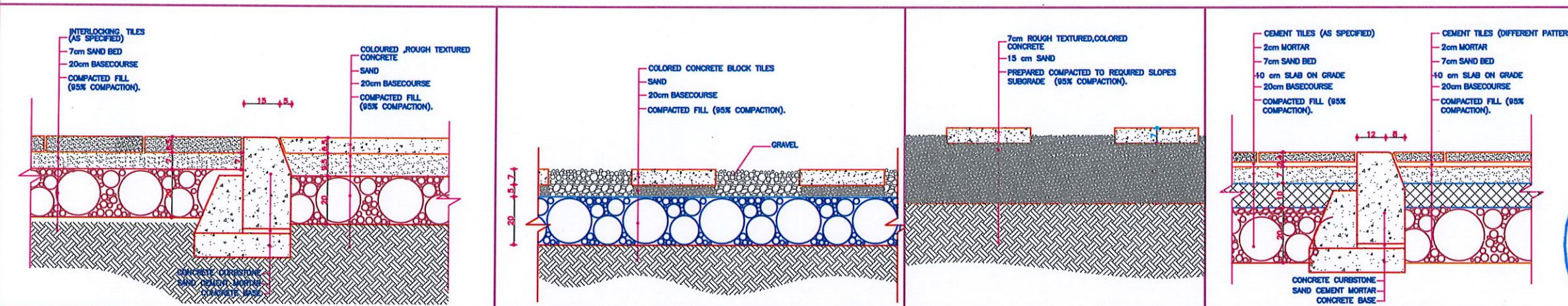
DET.8 INTERLOCKING ADJACENT TO CONCRETE PAVING scale 1:10 DET.9 CONCRETE PAVING ADJACENT TO GRAVEL FINISH scale 1:10 DET.10 CONCRETE PAVING ON SAND scale 1:10 DET.11 CEMENT TILES ADJACENT TO CEMENT TILES DIFFERENT PATTERN scale 1:10
