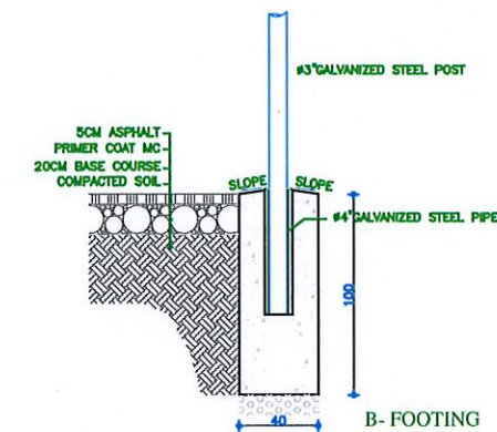
B- FOOTING
